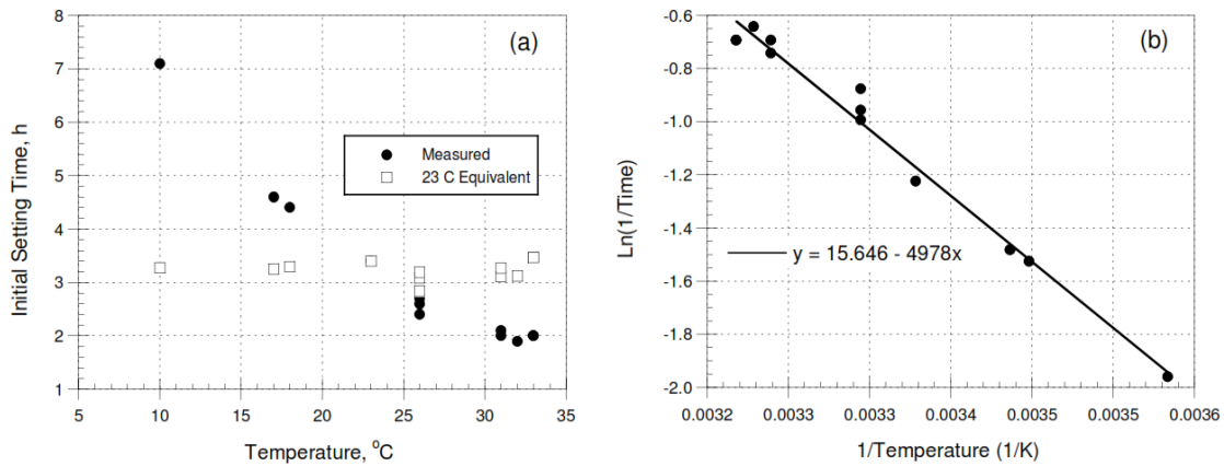
Figure 1. (a) Initial drtting time vs. temperature (b) inverse of setting time vs. inverse of absolute temperature (Pinto,R.C 1999)
